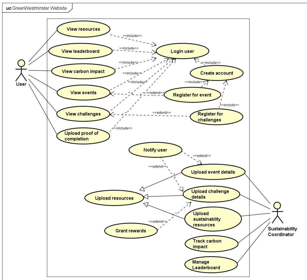
Figure 9 Earlier versions of Use case diagrams
