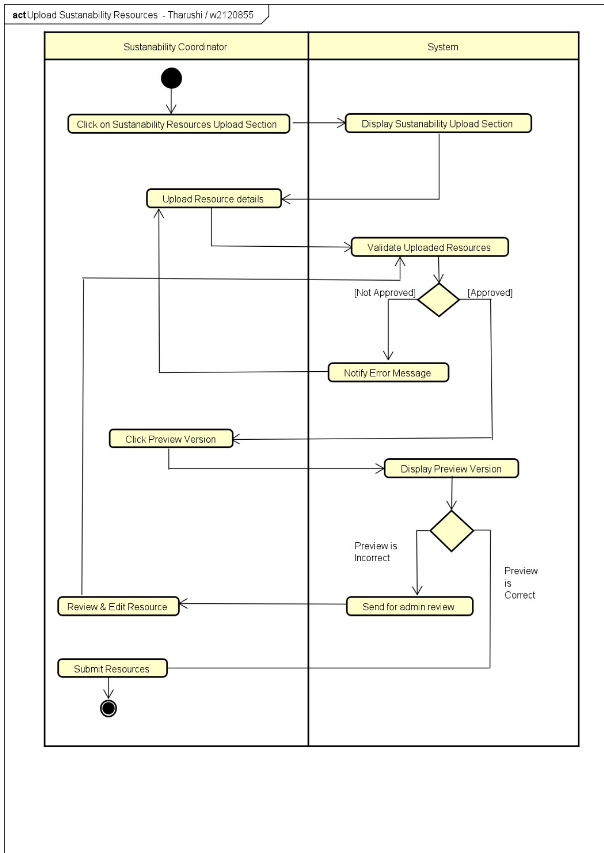
Figure 6 Activity Diagram for Upload sustainability resources
