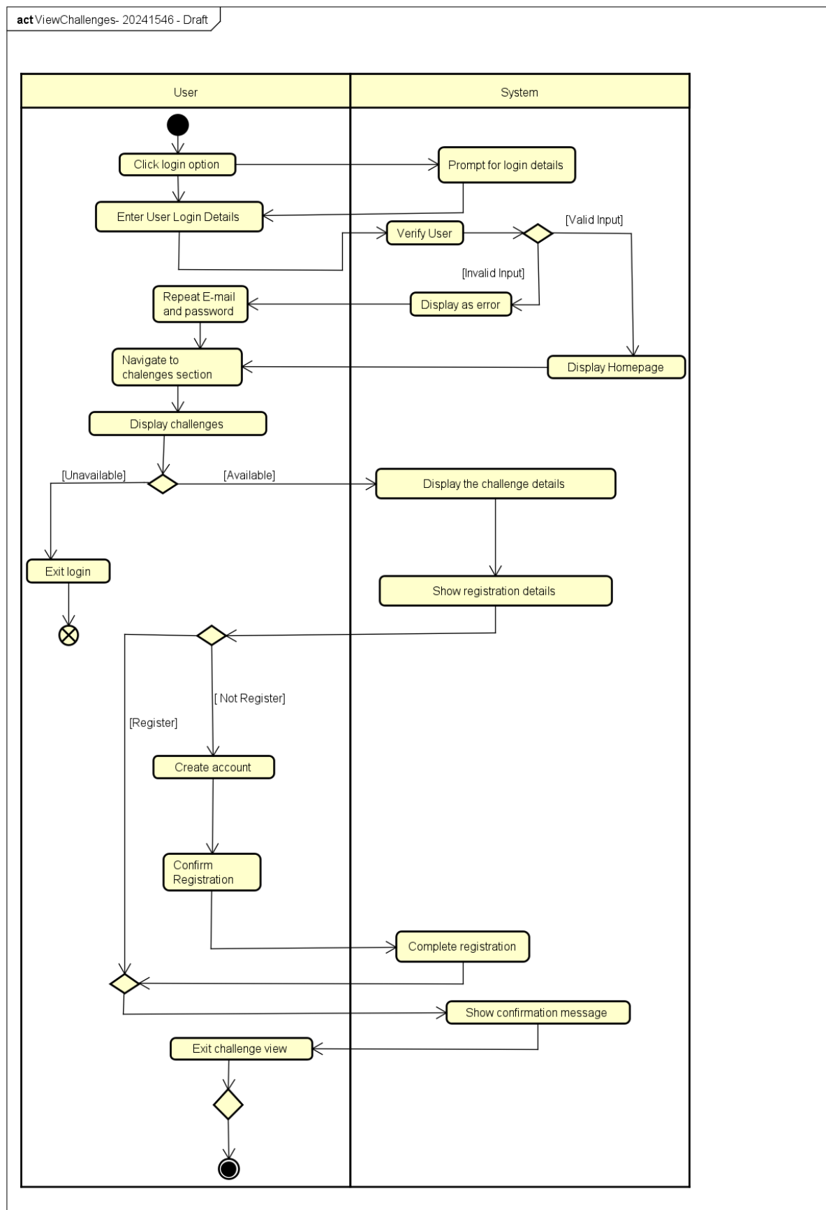
Figure 11 Earlier versions of Activity Diagram - View challenges.
