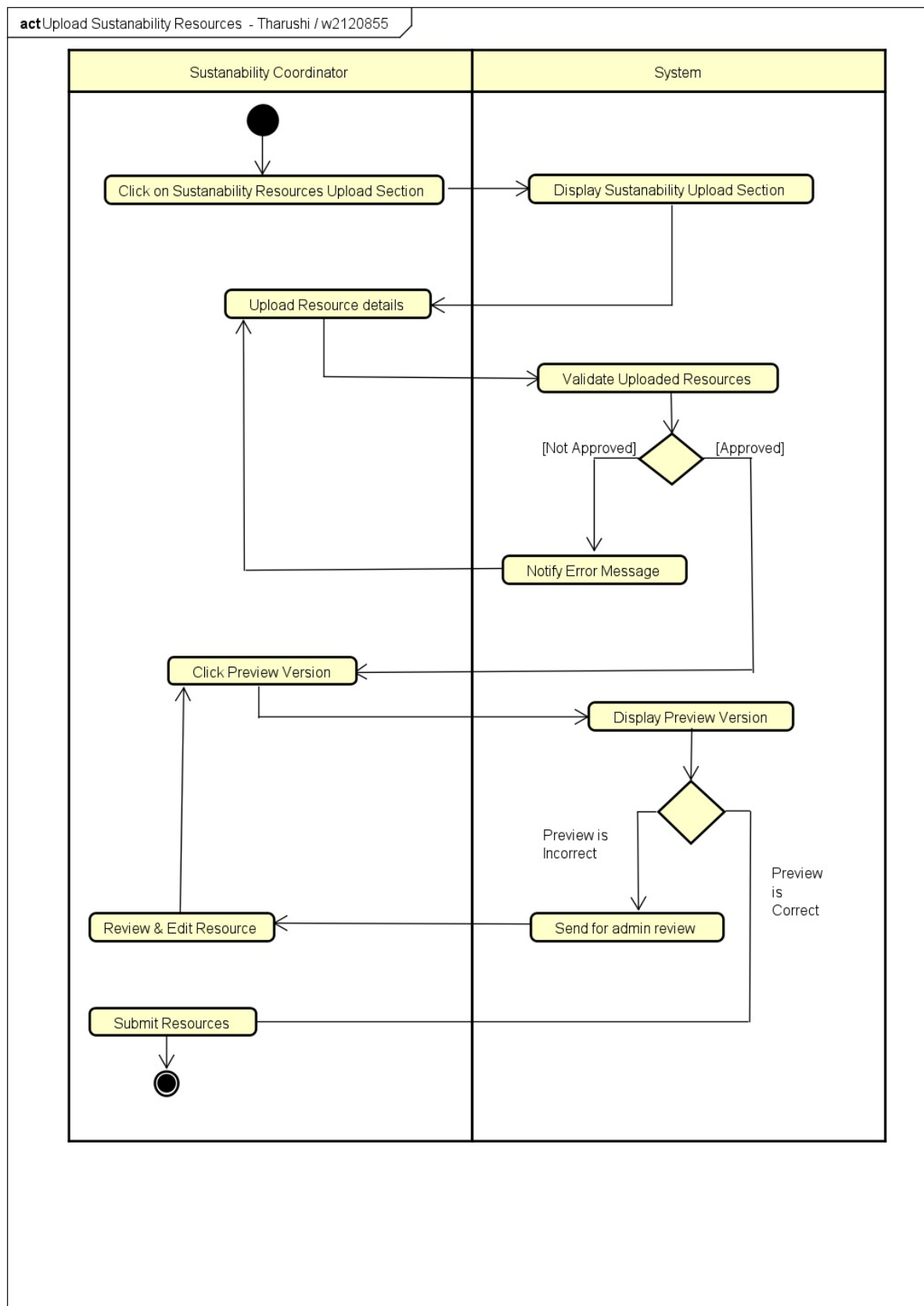
Figure 13 Earlier versions of Activity Diagram - Upload sustainability resources
