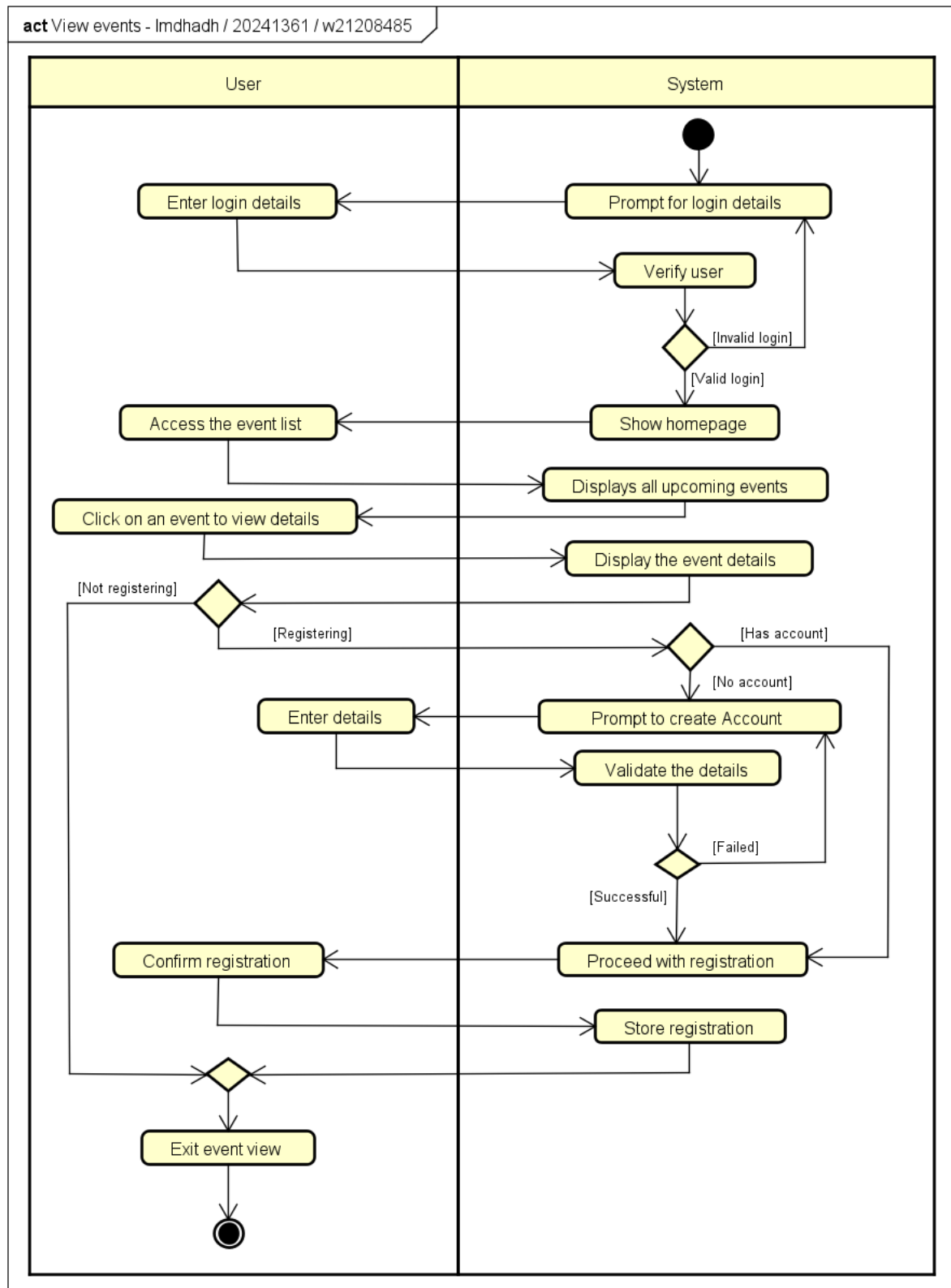
Figure 10 Earlier versions of Activity Diagram - View events
