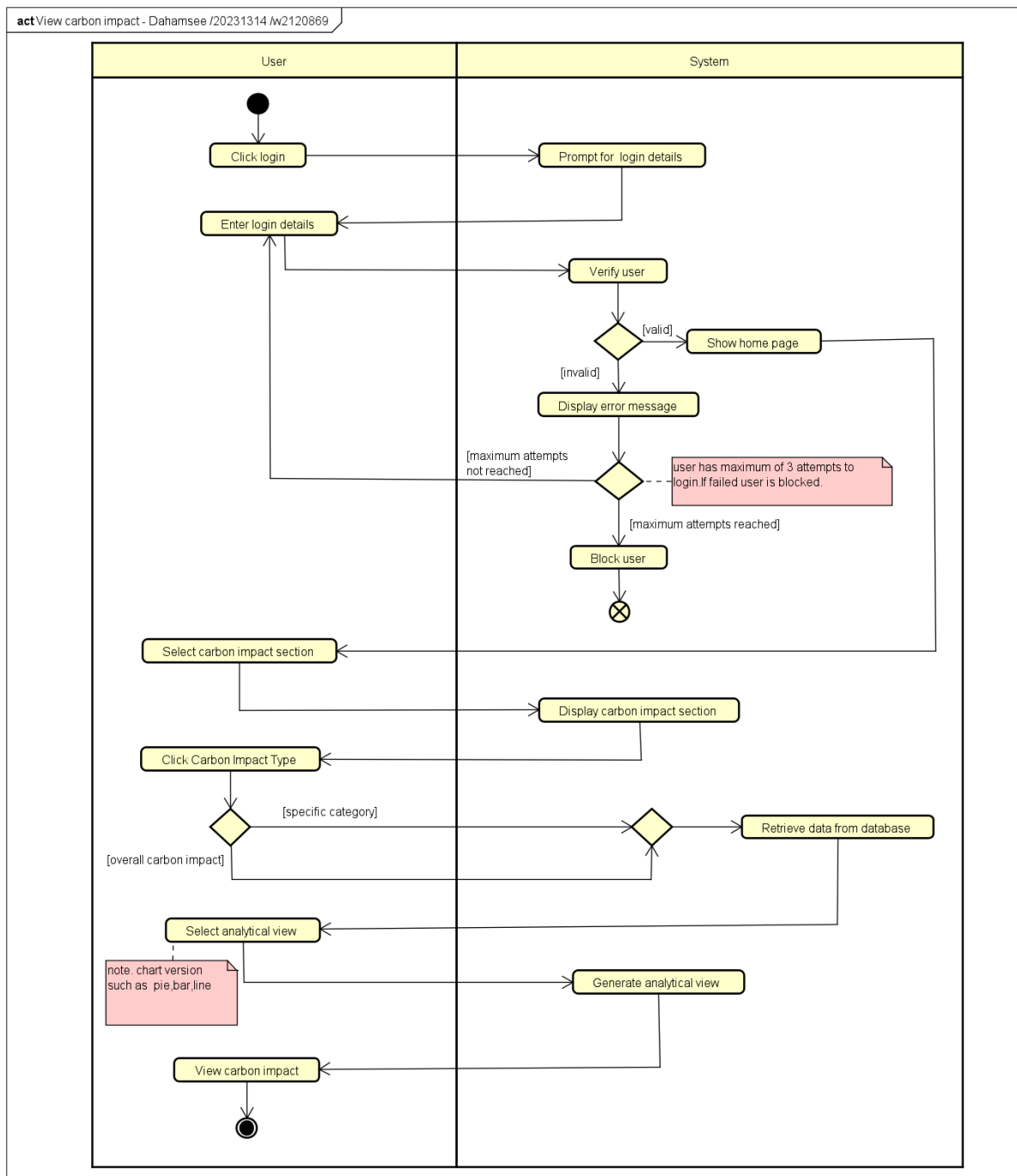
Figure 5 . Activity Diagram for View carbon impact
