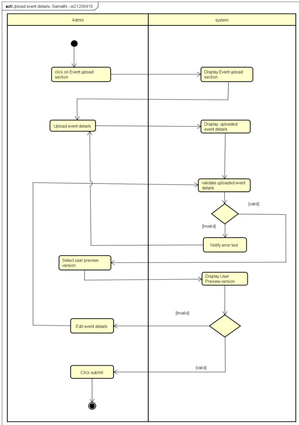
Figure 7 Activity Diagram for Upload event details
