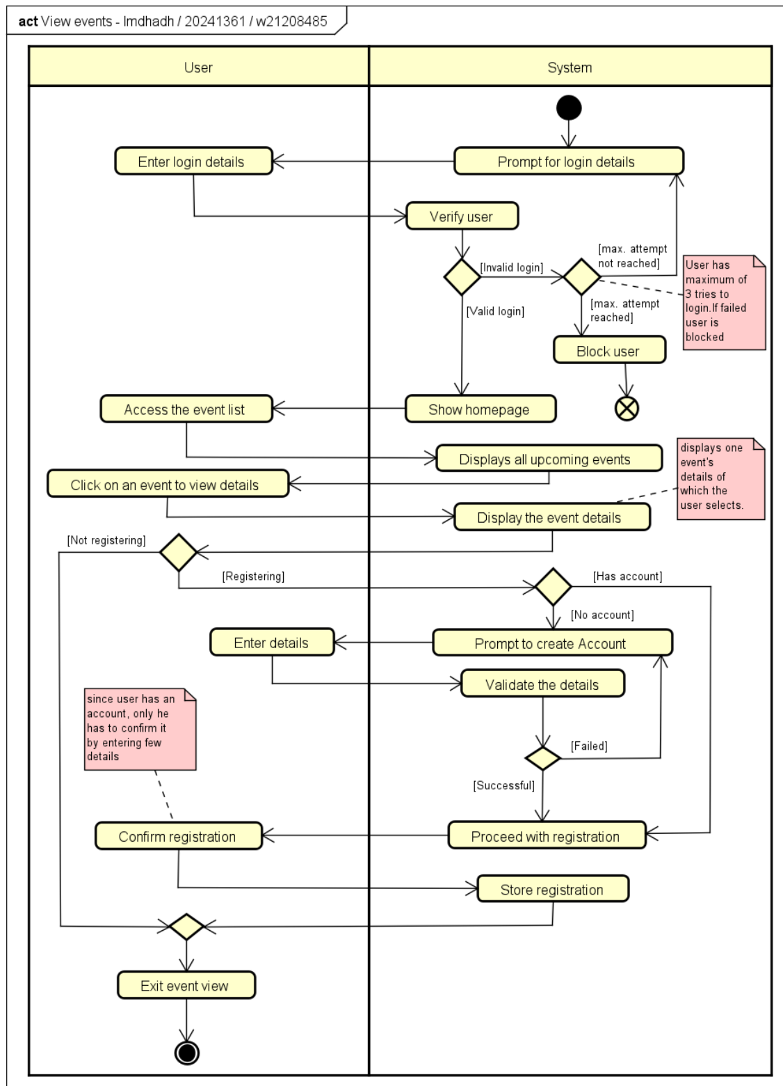
Figure 3 Activity Diagram for View events
